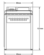
ODS-AGM15LMJ RIGHT POSITIVE FEMALE TERMINAL
